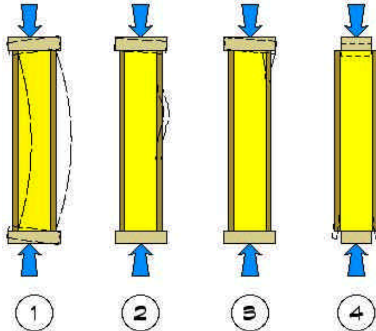
Figure 2: Failure modes for a load-bearing straw bale wall
